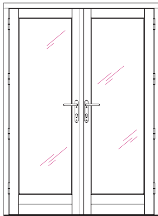
H101 Hi-Load Lift Off Hinge 4 Hinges Per Door Maximum Adjusted Door Weight 80kg
